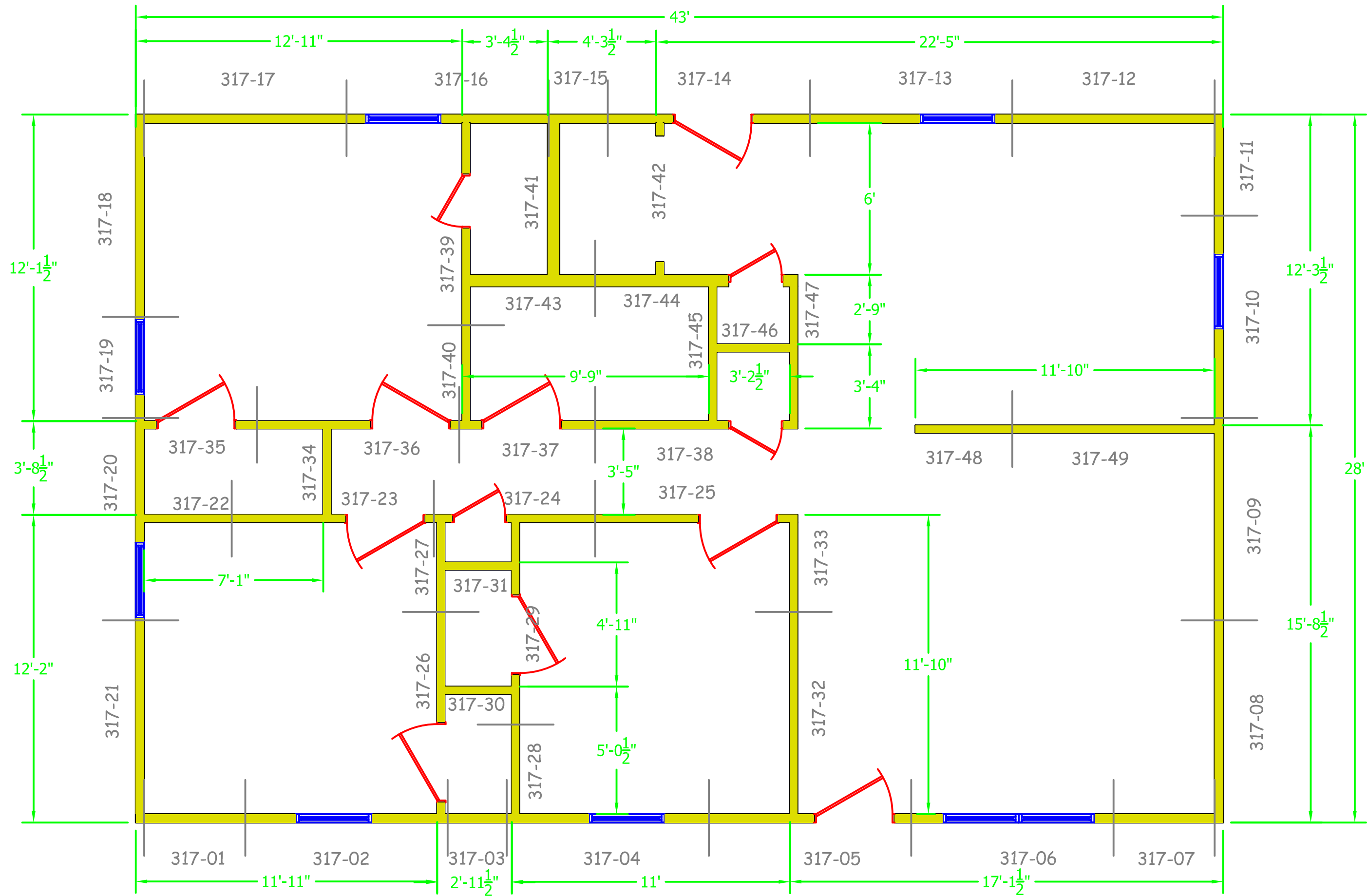
3 BEDROOM HOUSE 317
